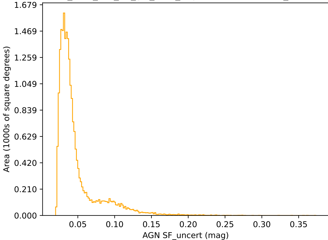
too_elab_r64_d3_giz_v3.4_10yrs r band: AGN SF_uncert
