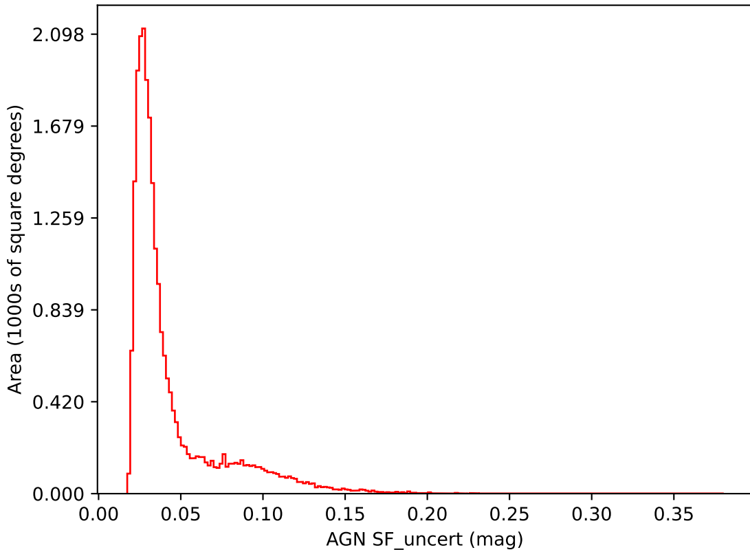
too_elab_r64_d3_giz_v3.4_10yrs i band: AGN SF_uncert
