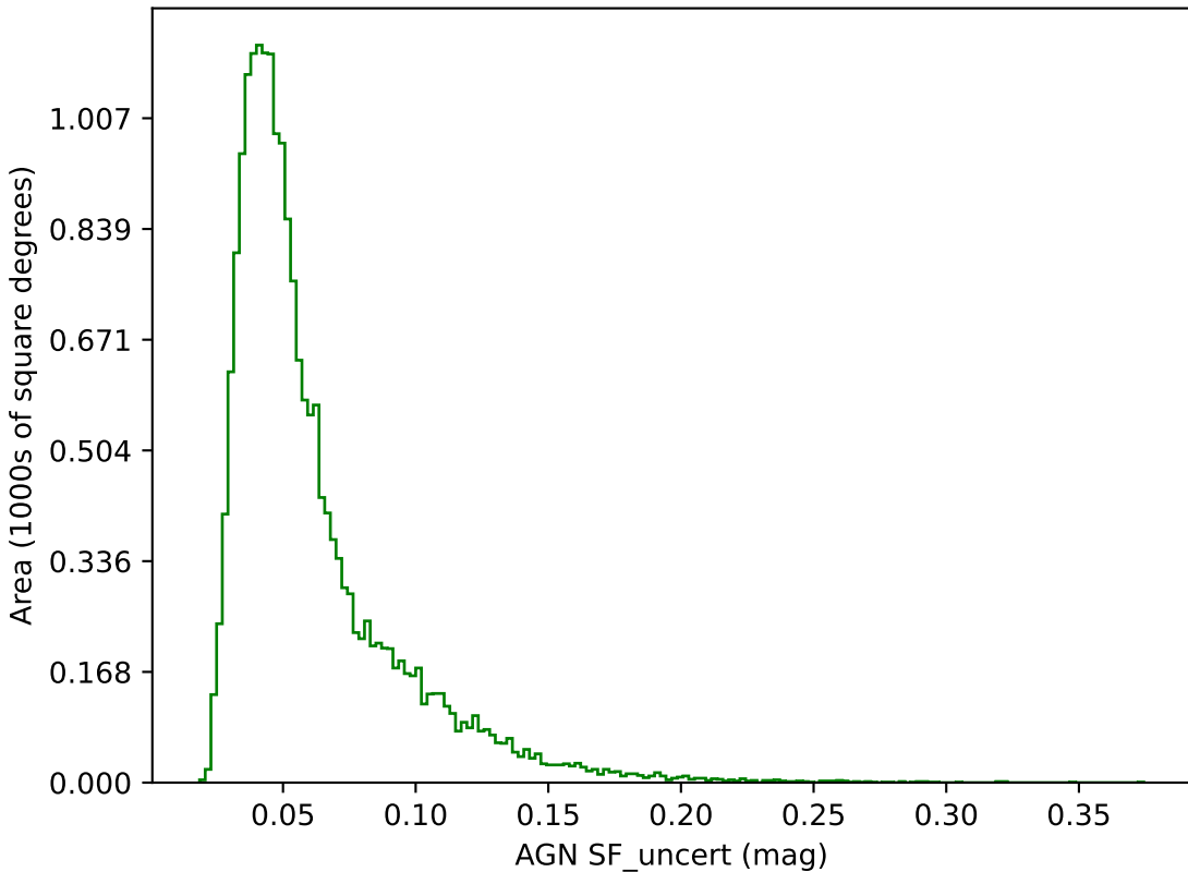
too_elab_r64_d3_giz_v3.4_10yrs g band: AGN SF_uncert
