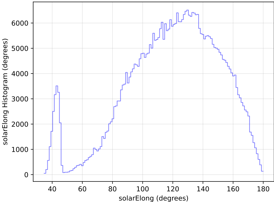
too_elab_r64_d3_giz_v3.4_10yrs WFD z band: solarElong Histogram
