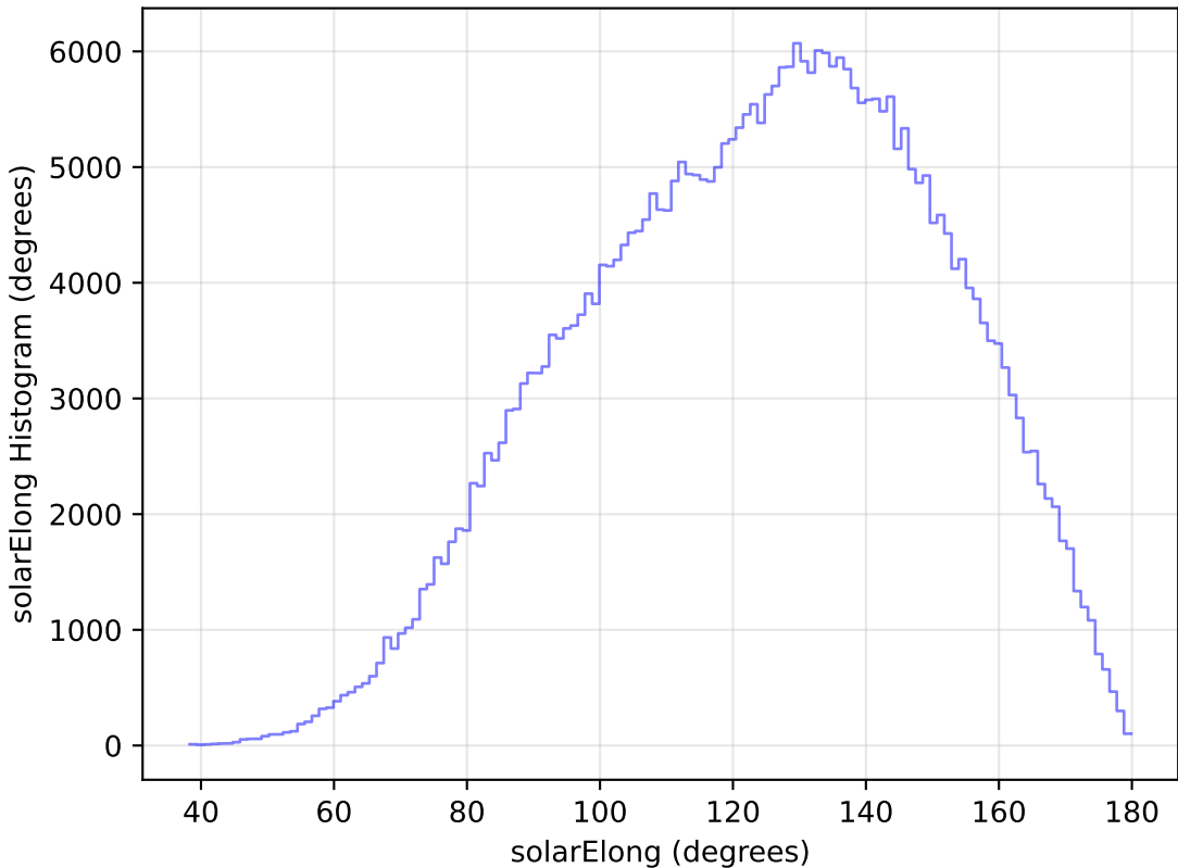
too_elab_r64_d3_giz_v3.4_10yrs WFD y band: solarElong Histogram
