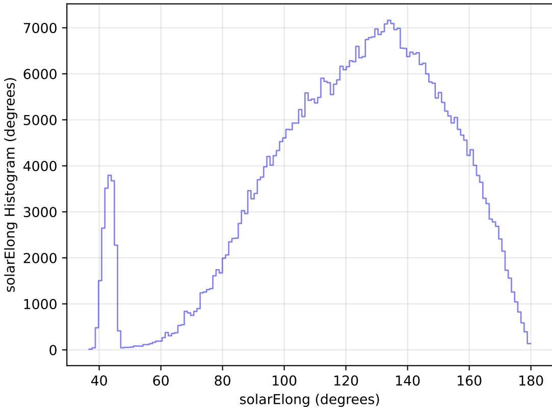
too_elab_r64_d3_giz_v3.4_10yrs WFD r band: solarElong Histogram
