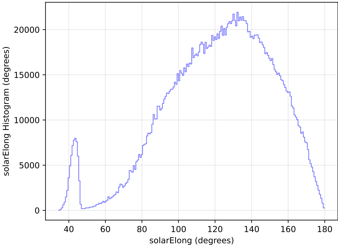
too_elab_r64_d3_giz_v3.4_10yrs WFD all bands: solarElong Histogram
