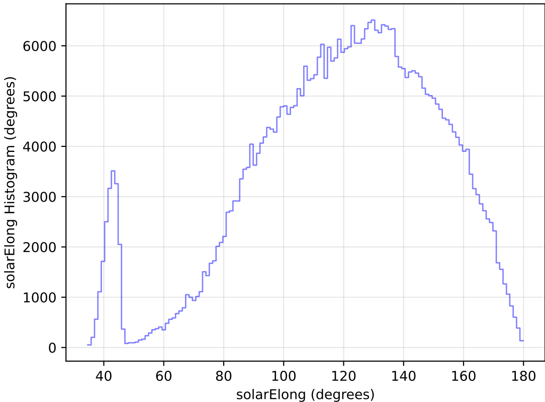
too_elab_r64_d3_giz_v3.4_10yrs All sky z band: solarElong Histogram
