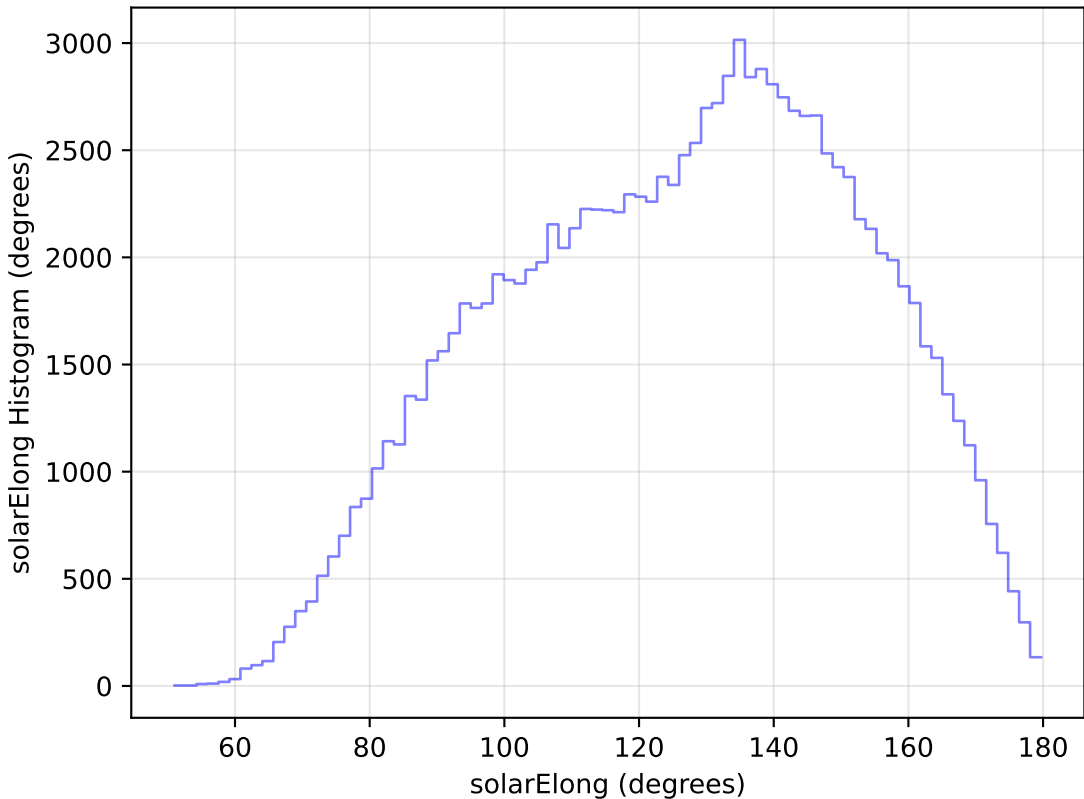
too_elab_r64_d3_giz_v3.4_10yrs All sky u band: solarElong Histogram
