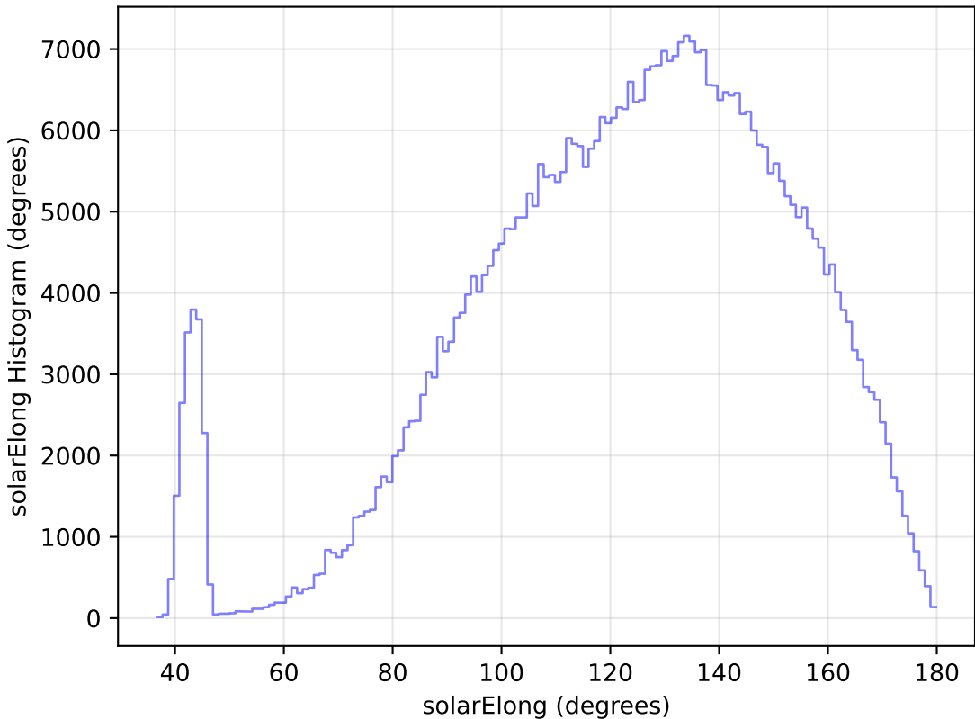
too_elab_r64_d3_giz_v3.4_10yrs All sky r band: solarElong Histogram
