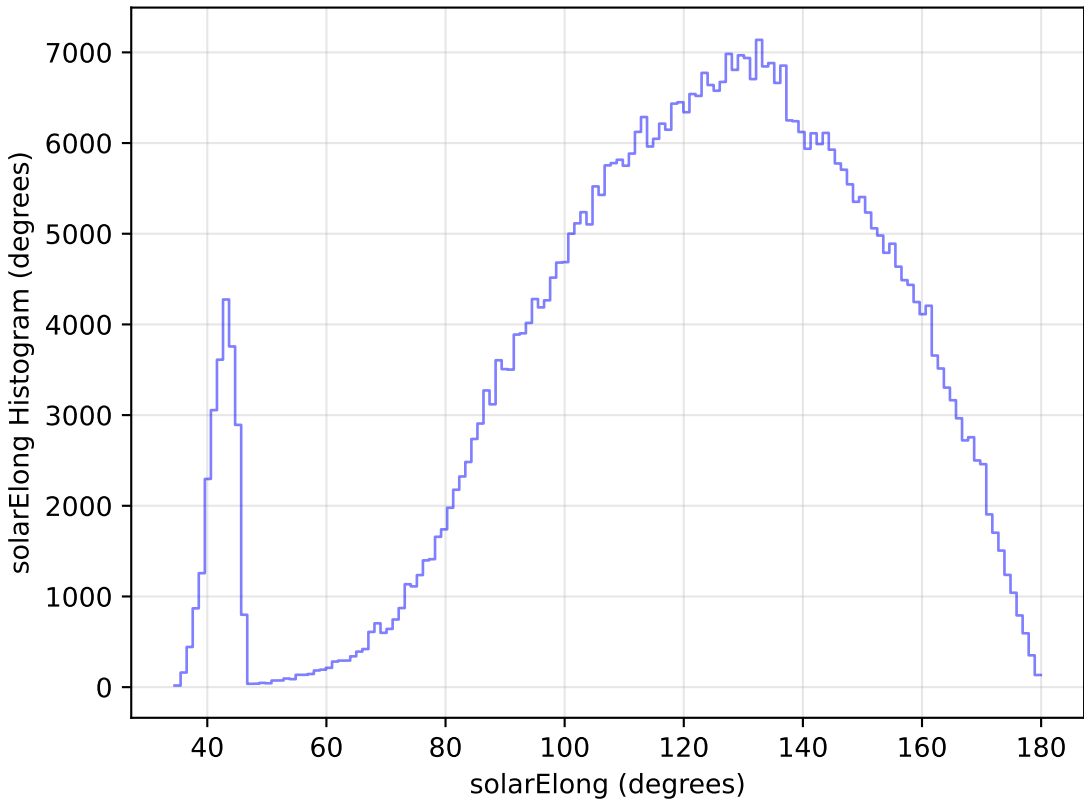
too_elab_r64_d3_giz_v3.4_10yrs All sky i band: solarElong Histogram
