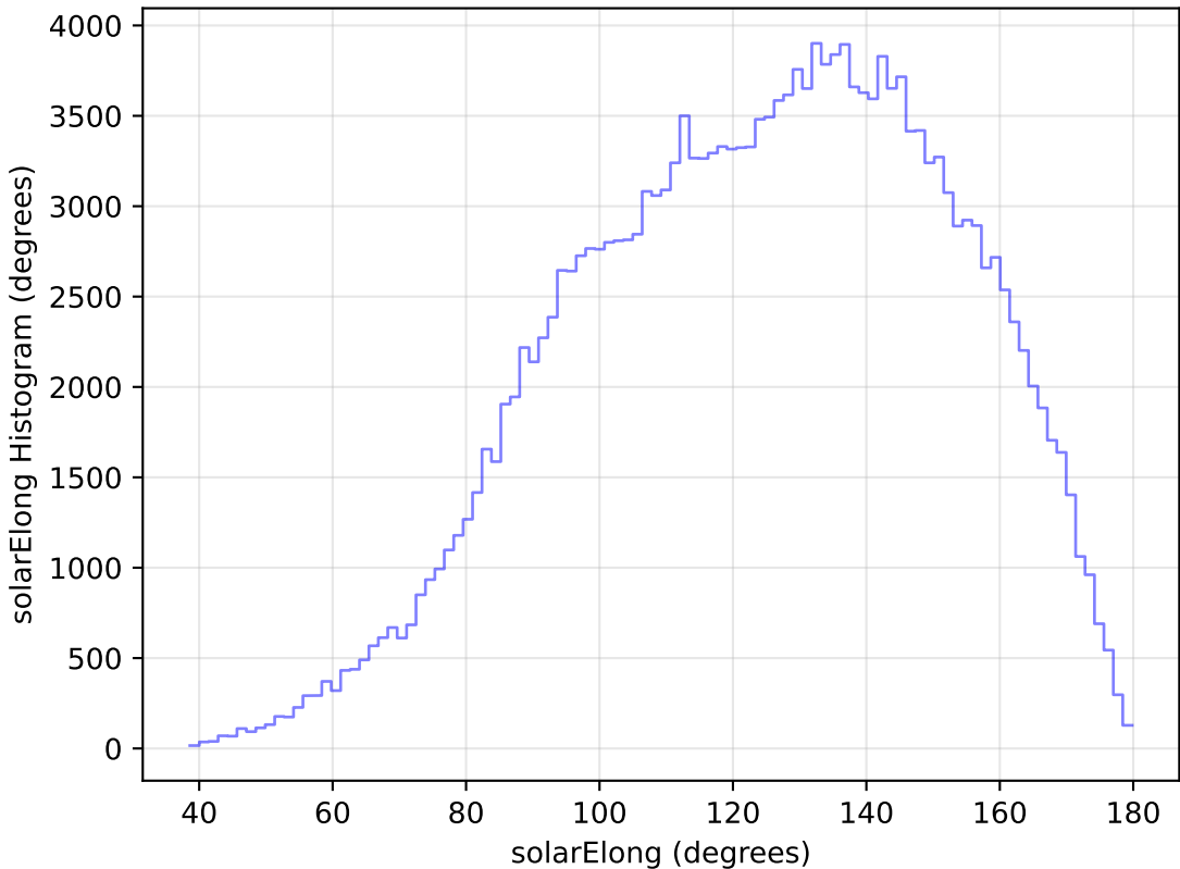
too_elab_r64_d3_giz_v3.4_10yrs All sky g band: solarElong Histogram
