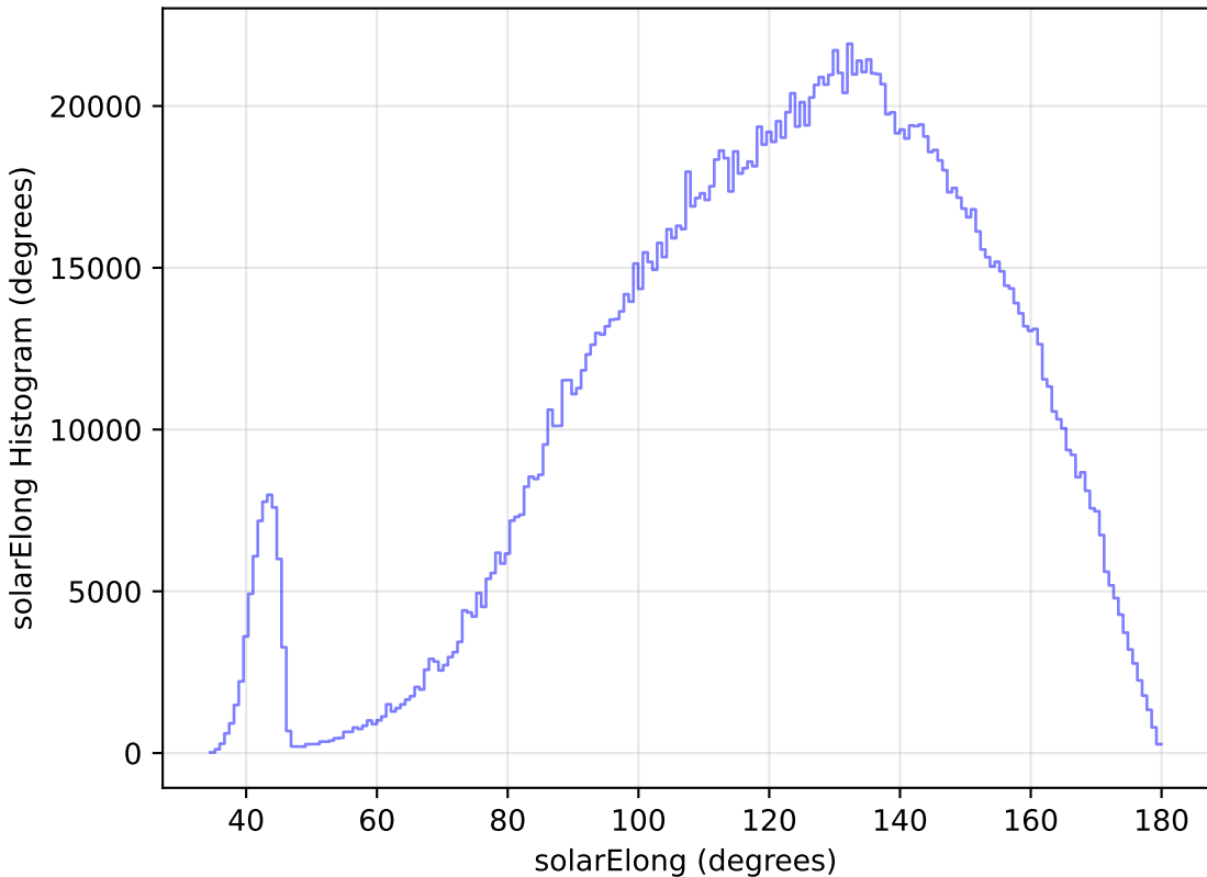
too_elab_r64_d3_giz_v3.4_10yrs All sky all bands: solarElong Histogram
