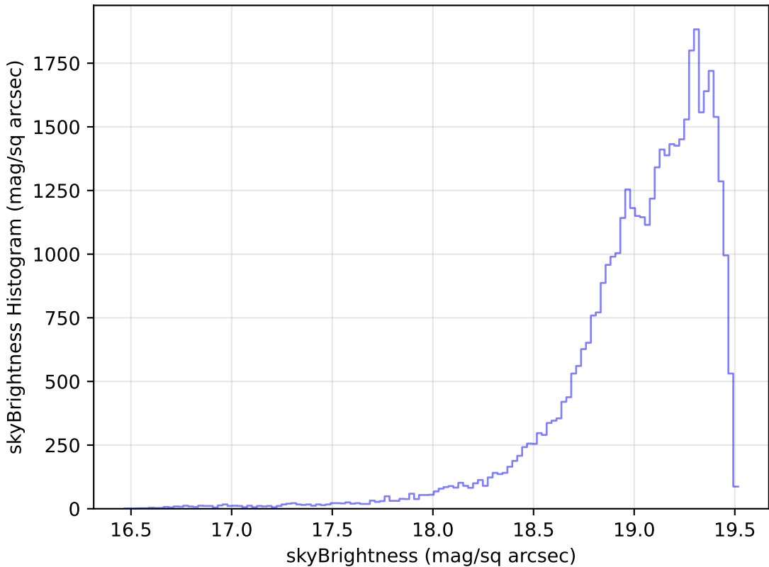
too_elab_r64_d3_giz_v3.4_10yrs Yr 1 z band: skyBrightness Histogram
