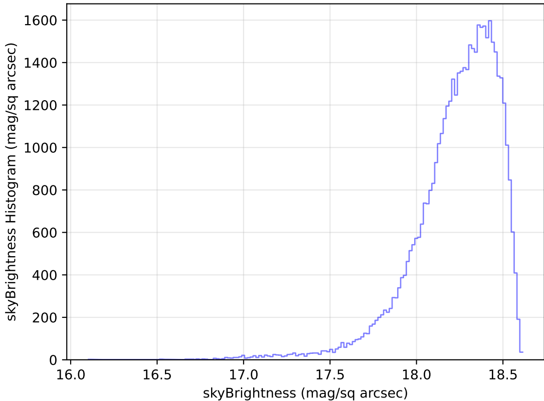
too_elab_r64_d3_giz_v3.4_10yrs Yr 1 y band: skyBrightness Histogram
