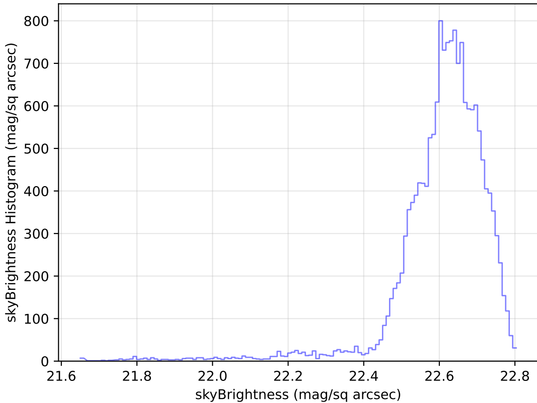
too_elab_r64_d3_giz_v3.4_10yrs Yr 1 u band: skyBrightness Histogram
