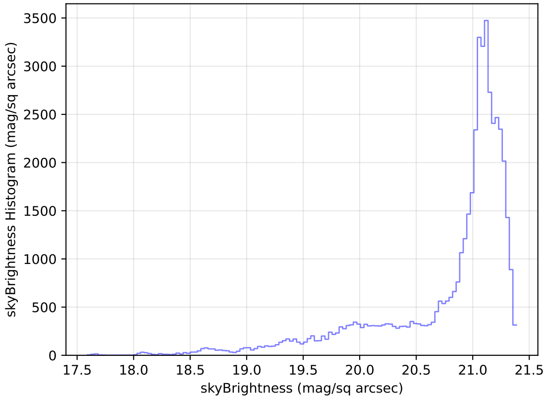
too_elab_r64_d3_giz_v3.4_10yrs Yr 1 r band: skyBrightness Histogram
