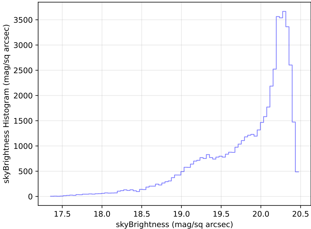
too_elab_r64_d3_giz_v3.4_10yrs Yr 1 i band: skyBrightness Histogram
