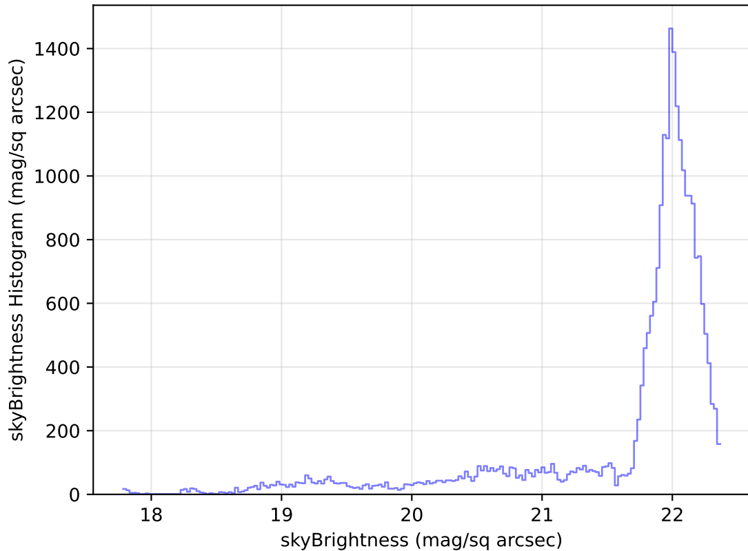
too_elab_r64_d3_giz_v3.4_10yrs Yr 1 g band: skyBrightness Histogram
