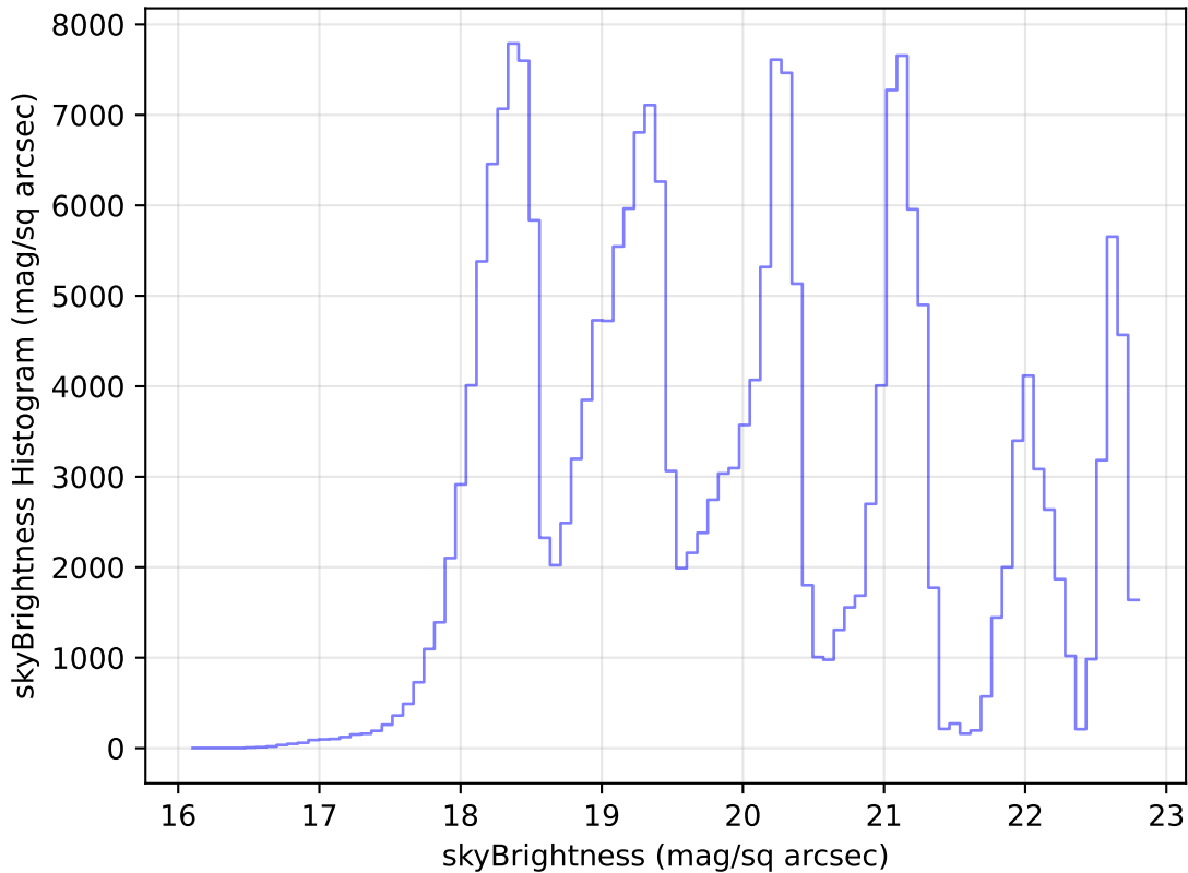
too_elab_r64_d3_giz_v3.4_10yrs Yr 1 all bands: skyBrightness Histogram
