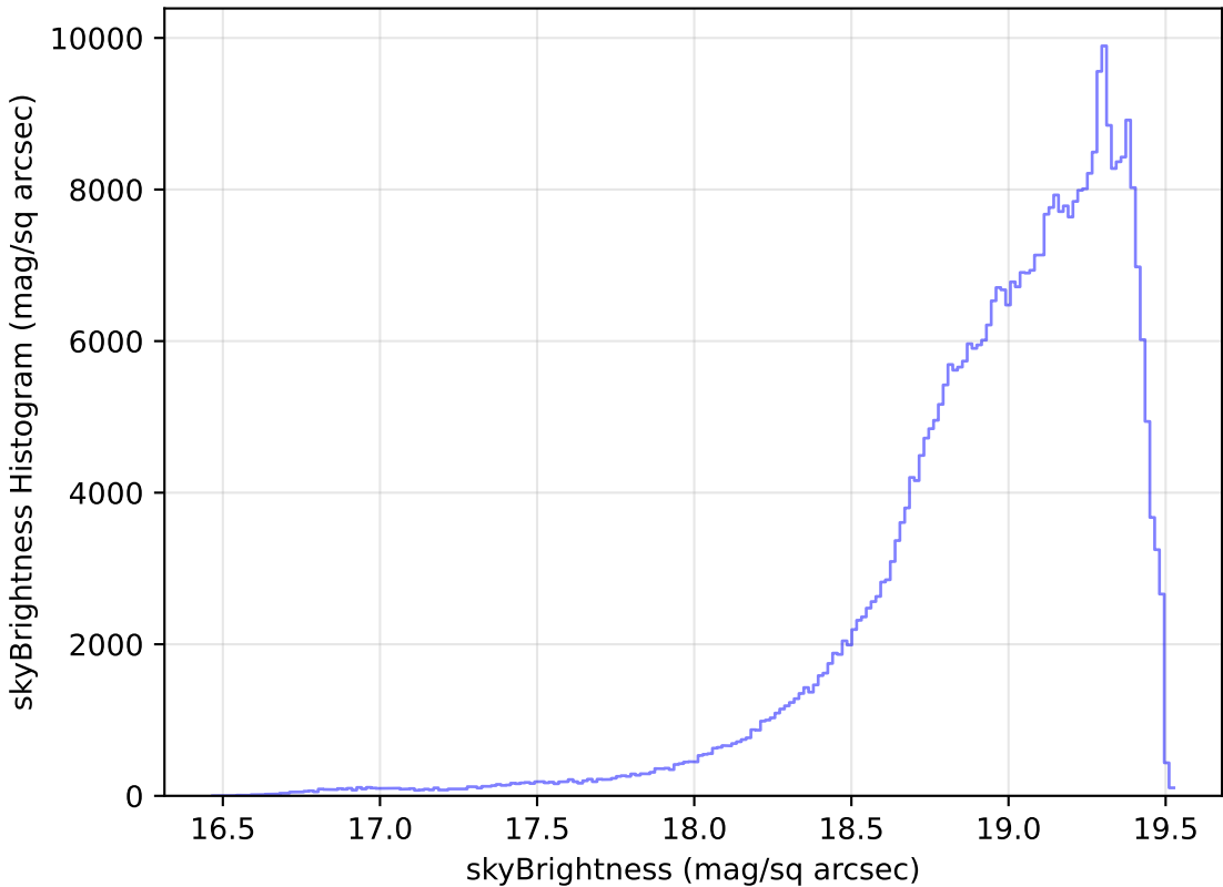
too_elab_r64_d3_giz_v3.4_10yrs WFD z band: skyBrightness Histogram
