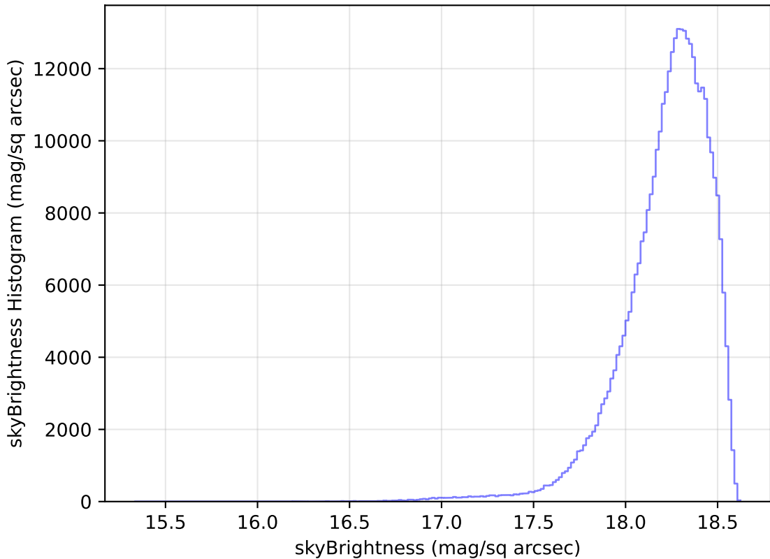
too_elab_r64_d3_giz_v3.4_10yrs WFD y band: skyBrightness Histogram
