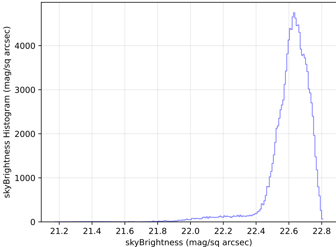
too_elab_r64_d3_giz_v3.4_10yrs WFD u band: skyBrightness Histogram
