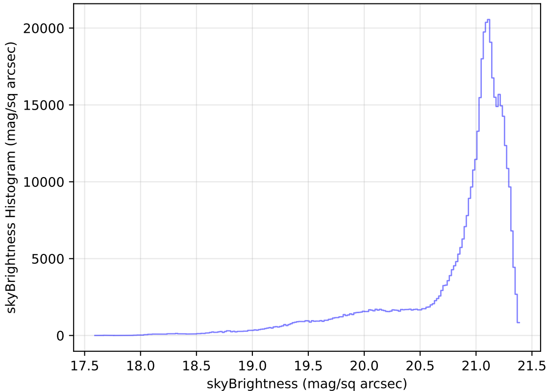
too_elab_r64_d3_giz_v3.4_10yrs WFD r band: skyBrightness Histogram
