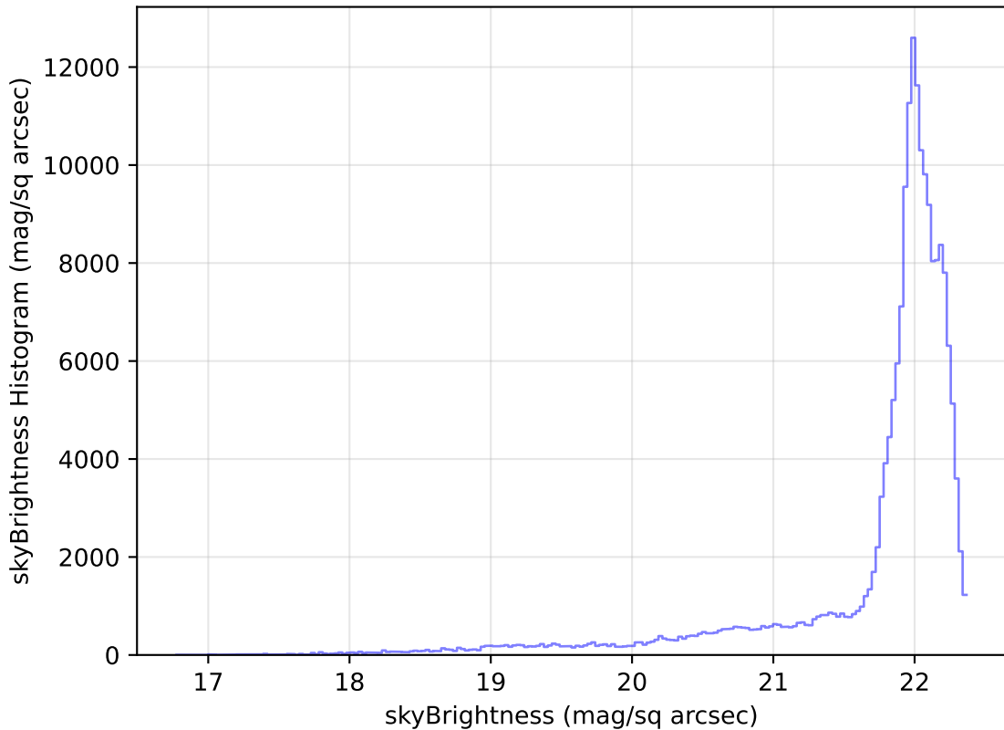
too_elab_r64_d3_giz_v3.4_10yrs WFD g band: skyBrightness Histogram
