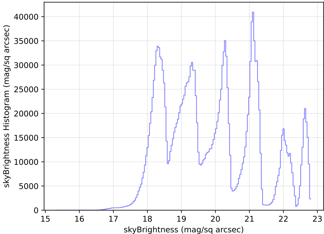
too_elab_r64_d3_giz_v3.4_10yrs WFD all bands: skyBrightness Histogram
