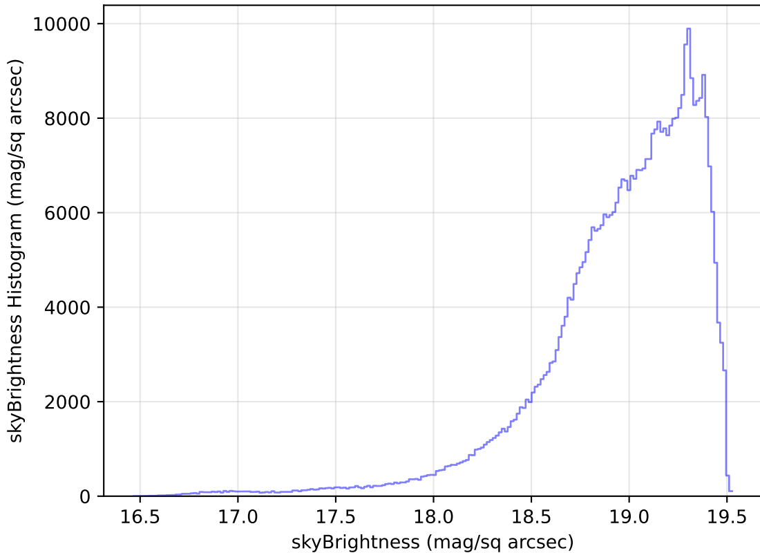
too_elab_r64_d3_giz_v3.4_10yrs All sky z band: skyBrightness Histogram
