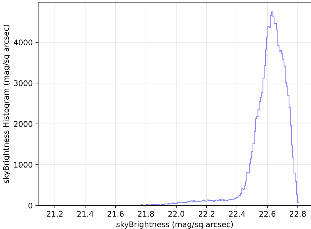
too_elab_r64_d3_giz_v3.4_10yrs All sky u band: skyBrightness Histogram
