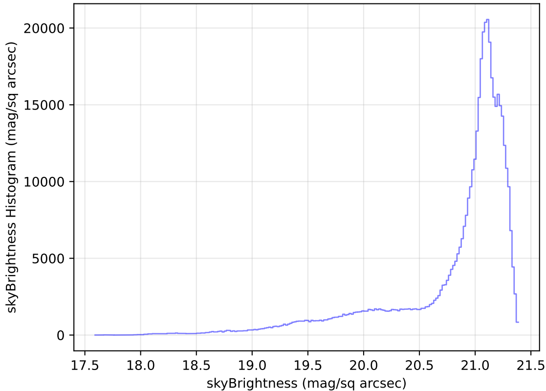
too_elab_r64_d3_giz_v3.4_10yrs All sky r band: skyBrightness Histogram
