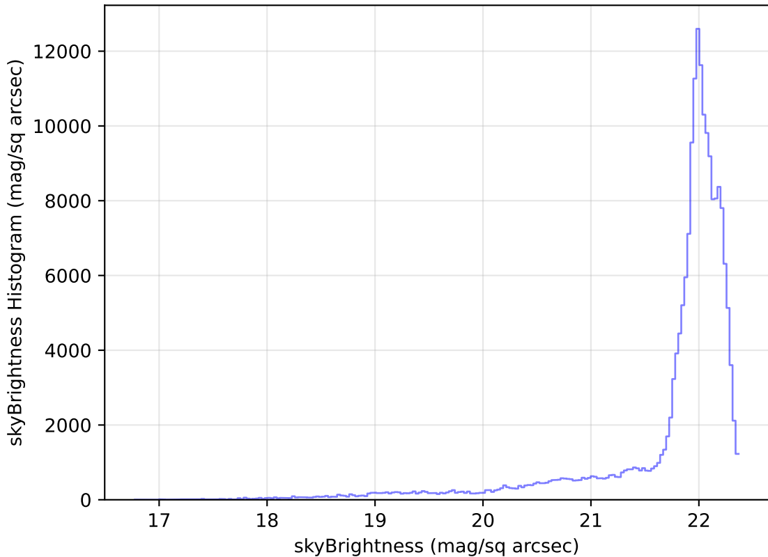
too_elab_r64_d3_giz_v3.4_10yrs All sky g band: skyBrightness Histogram
