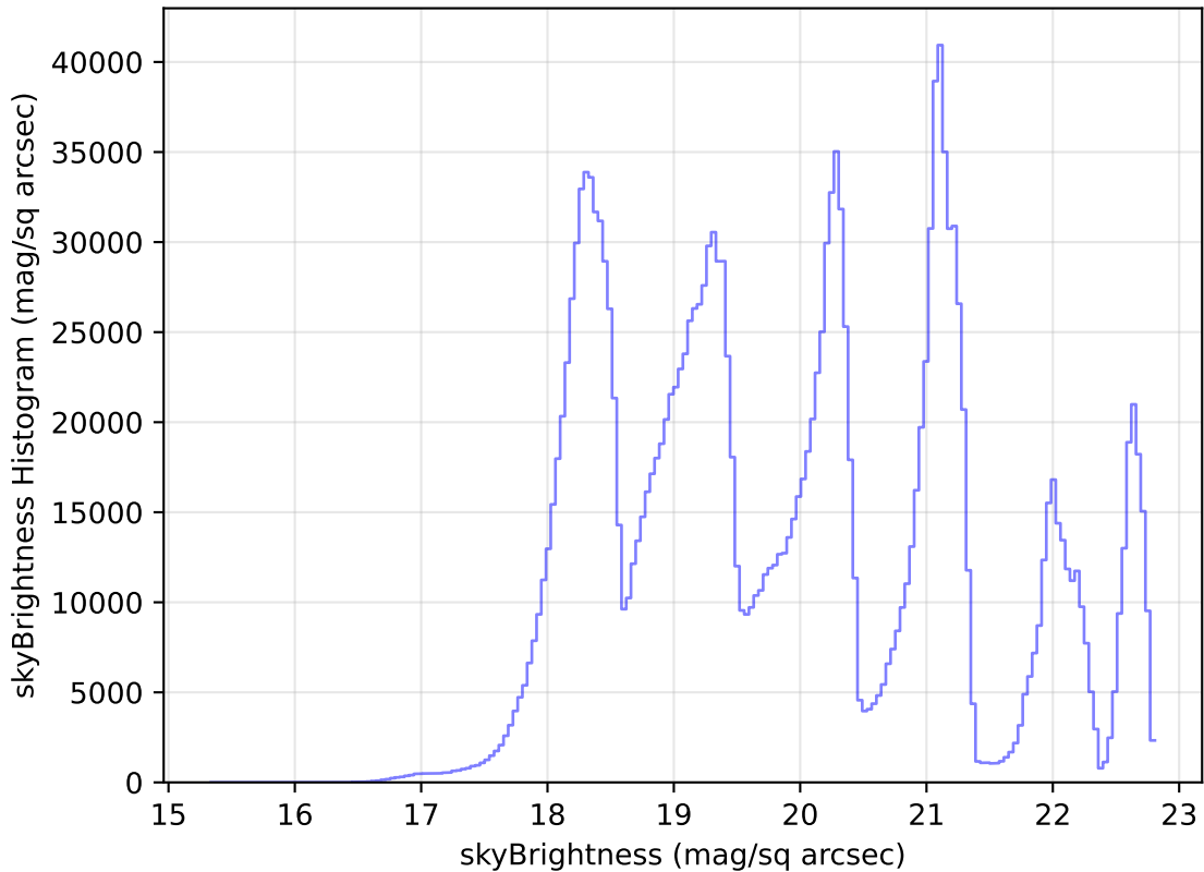
too_elab_r64_d3_giz_v3.4_10yrs All sky all bands: skyBrightness Histogram
