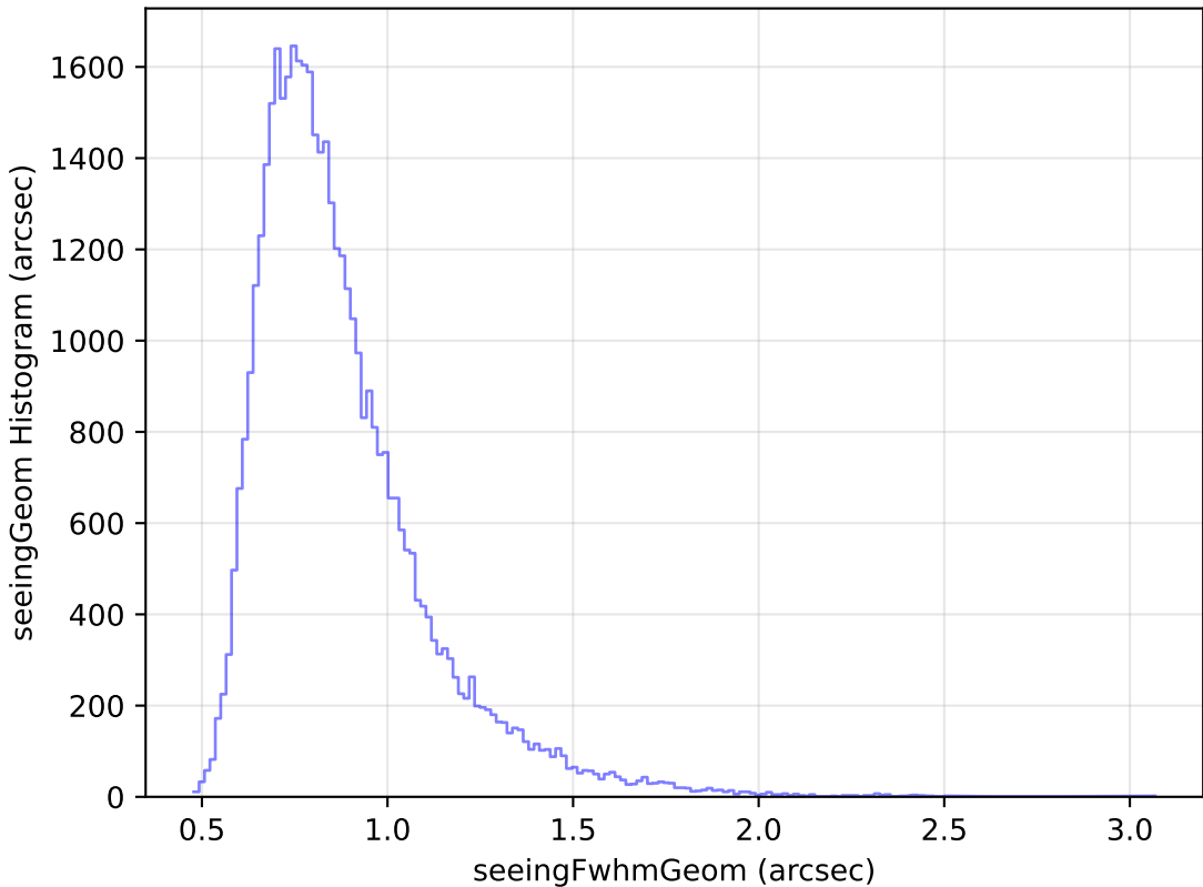
too_elab_r64_d3_giz_v3.4_10yrs Yr 1 z band: seeingGeom Histogram
