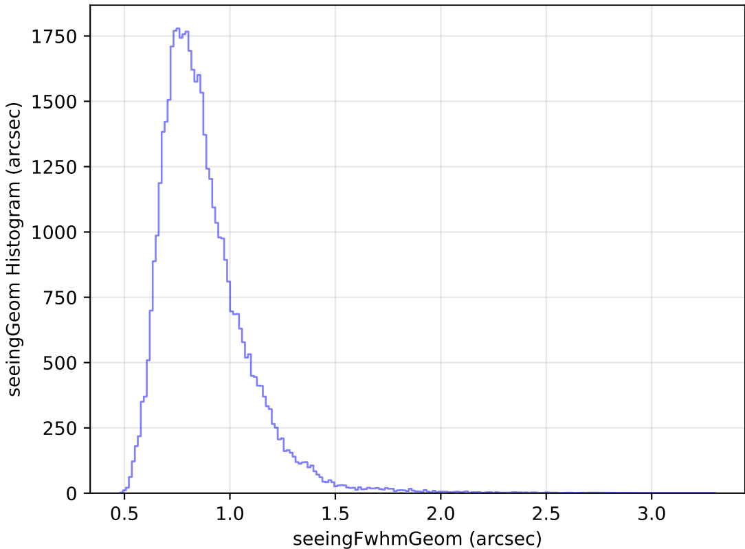
too_elab_r64_d3_giz_v3.4_10yrs Yr 1 y band: seeingGeom Histogram
