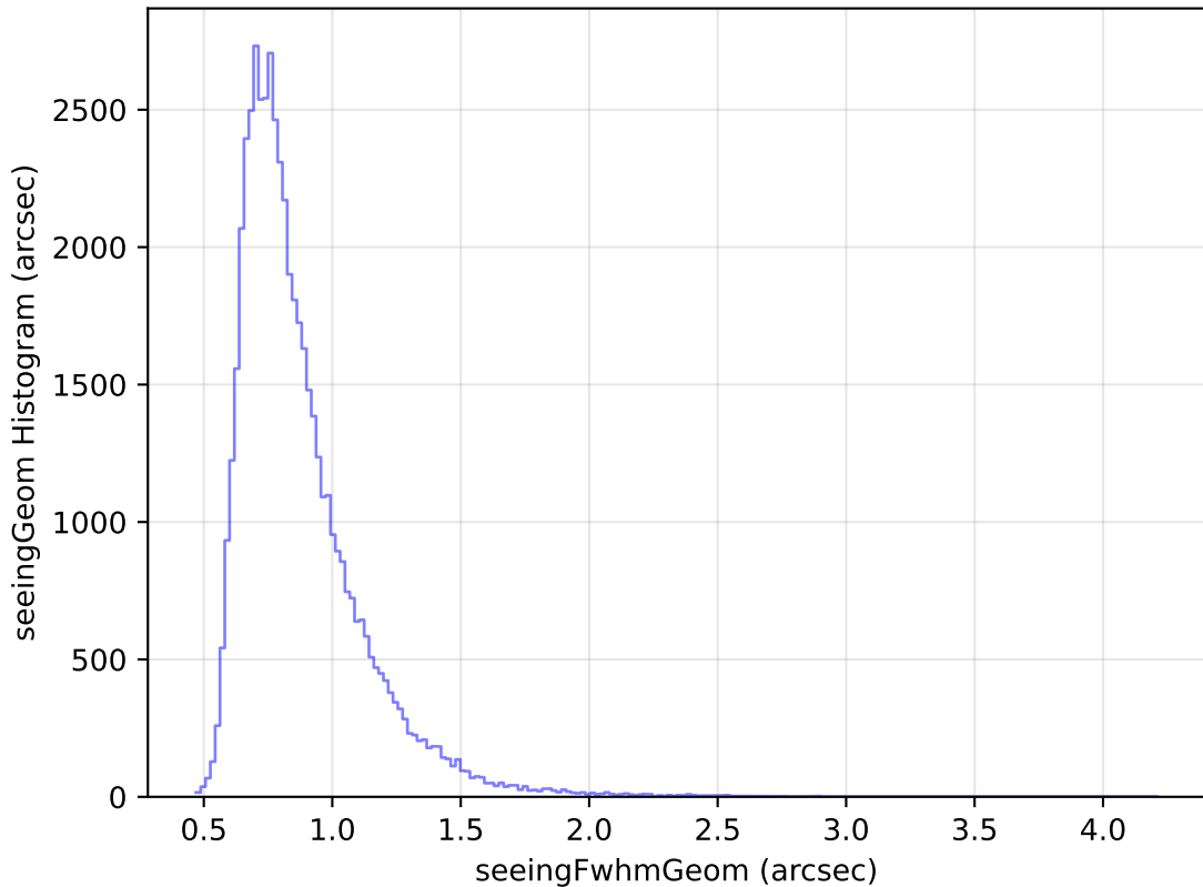
too_elab_r64_d3_giz_v3.4_10yrs Yr 1 i band: seeingGeom Histogram
