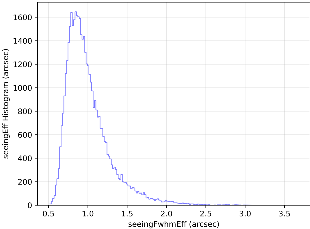
too_elab_r64_d3_giz_v3.4_10yrs Yr 1 z band: seeingEff Histogram
