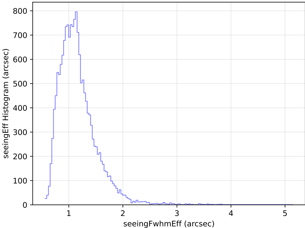
too_elab_r64_d3_giz_v3.4_10yrs Yr 1 u band: seeingEff Histogram
