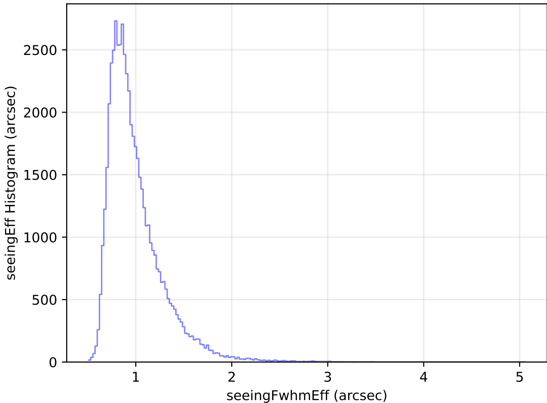
too_elab_r64_d3_giz_v3.4_10yrs Yr 1 i band: seeingEff Histogram
