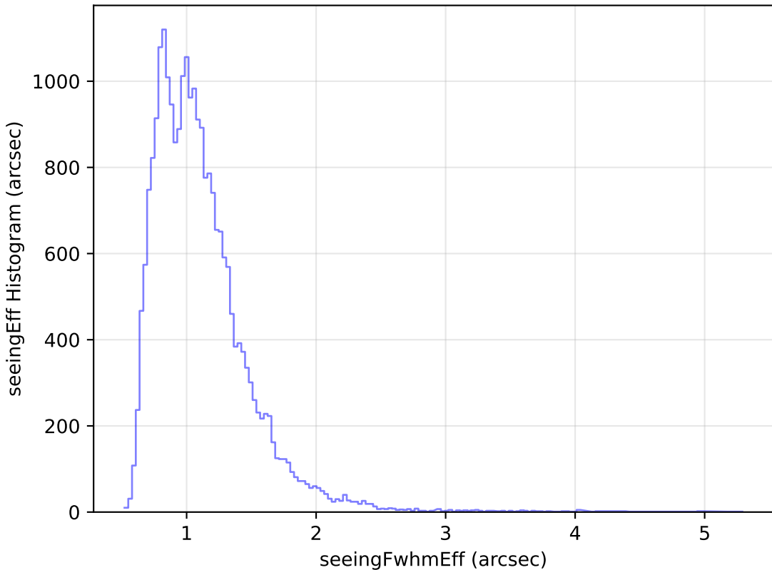
too_elab_r64_d3_giz_v3.4_10yrs Yr 1 g band: seeingEff Histogram
