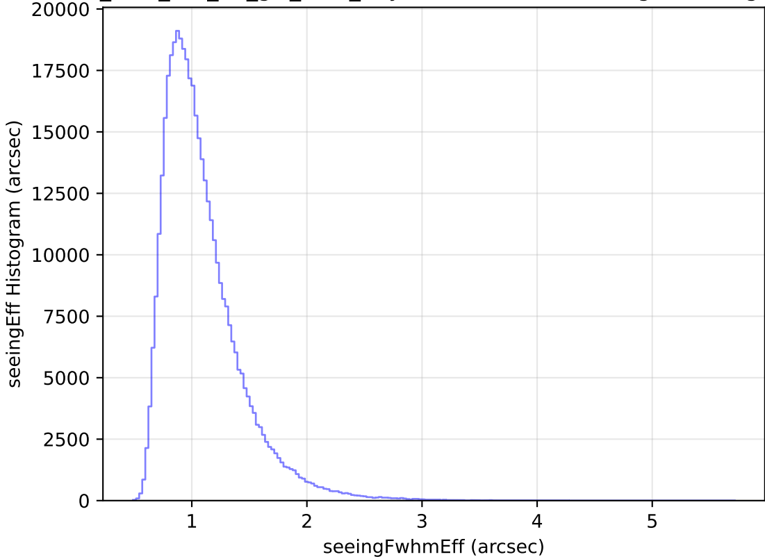
too_elab_r64_d3_giz_v3.4_10yrs WFD z band: seeingEff Histogram
