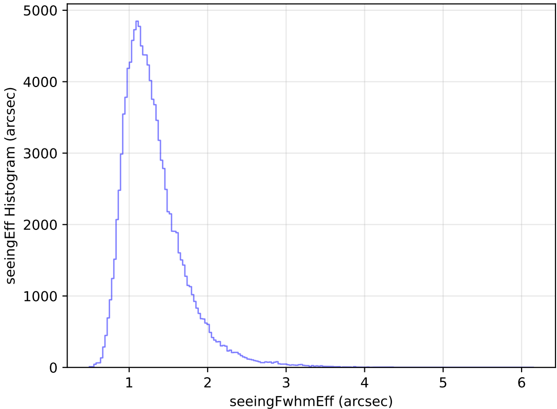
too_elab_r64_d3_giz_v3.4_10yrs WFD u band: seeingEff Histogram
