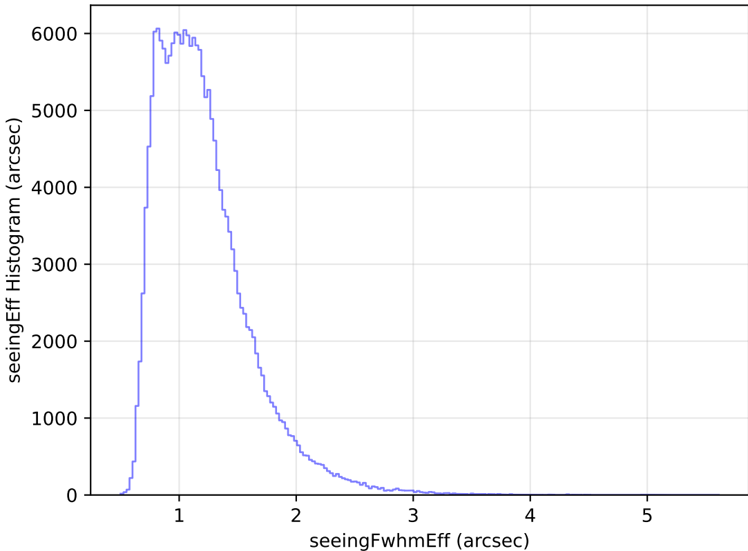
too_elab_r64_d3_giz_v3.4_10yrs WFD g band: seeingEff Histogram
