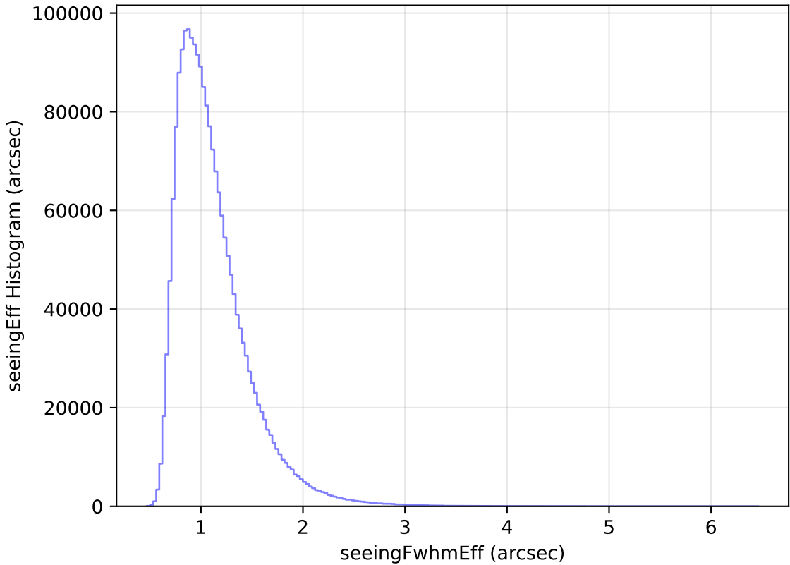
too_elab_r64_d3_giz_v3.4_10yrs WFD all bands: seeingEff Histogram
