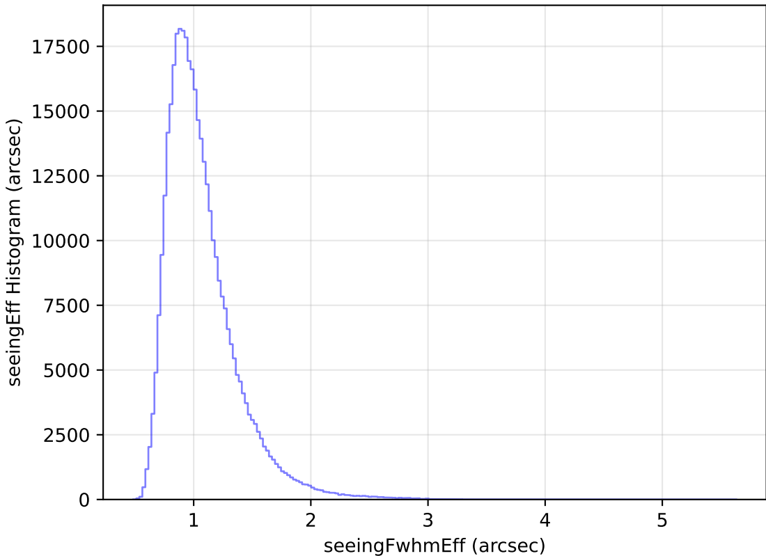
too_elab_r64_d3_giz_v3.4_10yrs All sky y band: seeingEff Histogram
