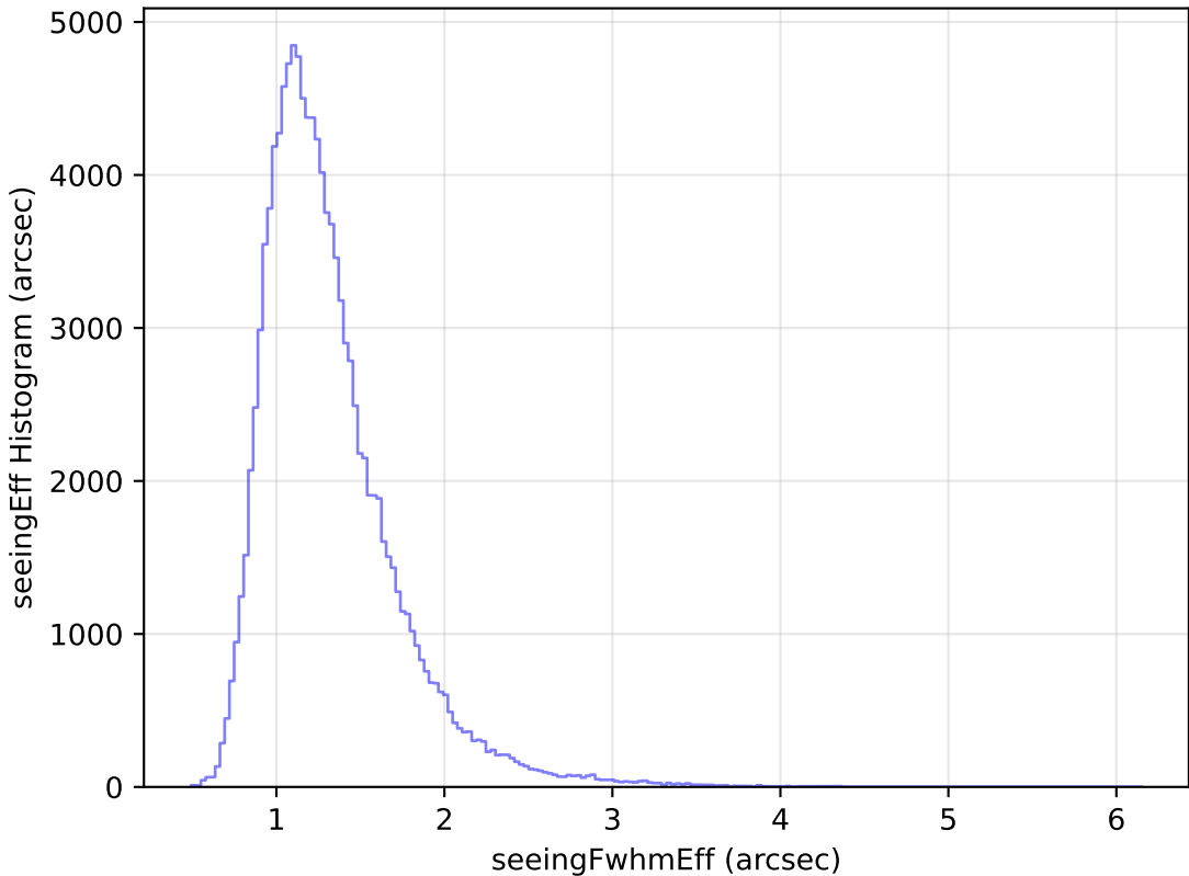
too_elab_r64_d3_giz_v3.4_10yrs All sky u band: seeingEff Histogram
