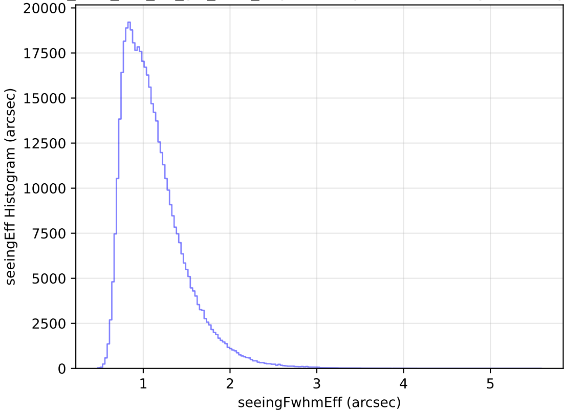
too_elab_r64_d3_giz_v3.4_10yrs All sky r band: seeingEff Histogram
