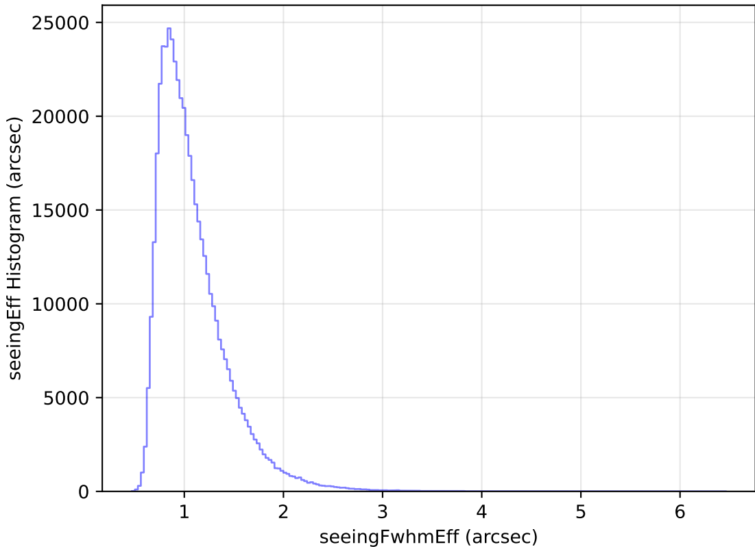
too_elab_r64_d3_giz_v3.4_10yrs All sky i band: seeingEff Histogram
