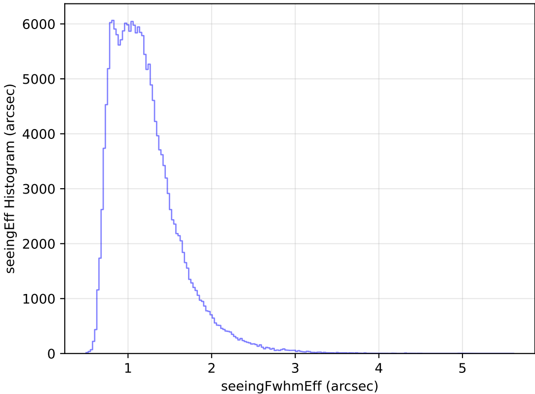
too_elab_r64_d3_giz_v3.4_10yrs All sky g band: seeingEff Histogram
