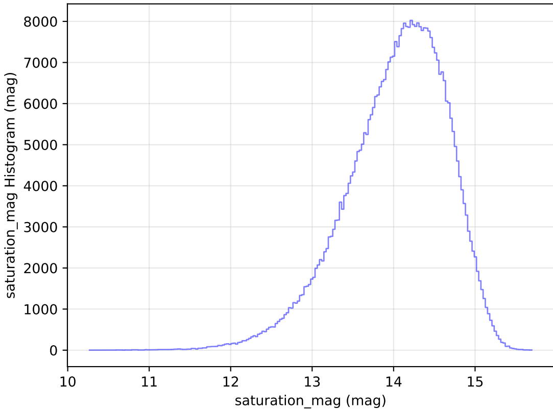
too_elab_r64_d3_giz_v3.4_10yrs WFD z band: saturation_mag Histogram
