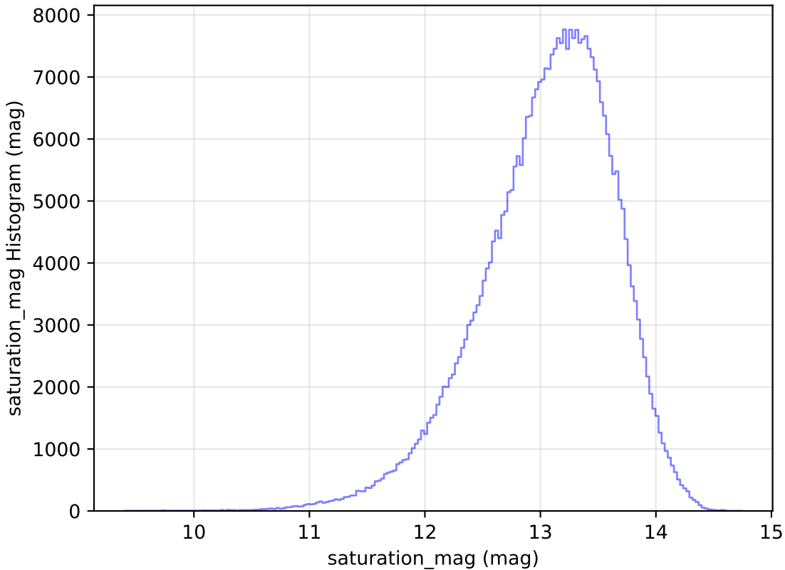
too_elab_r64_d3_giz_v3.4_10yrs WFD y band: saturation_mag Histogram
