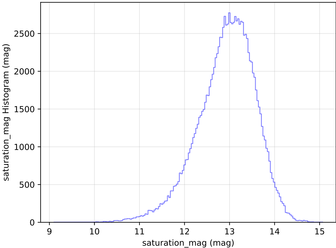
too_elab_r64_d3_giz_v3.4_10yrs WFD u band: saturation_mag Histogram
